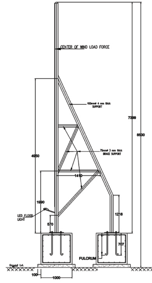
SECTIONAL ELEVATION
