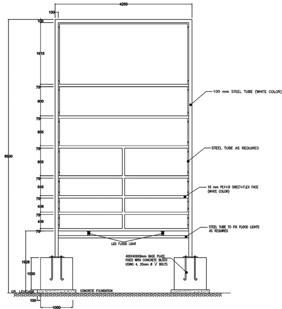
FRONT ELEVATION
